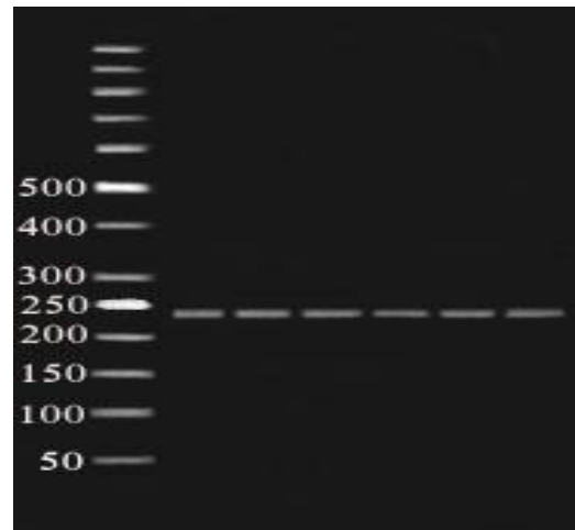
Figure 6. Fragments (48, 227bp) of AluI enzyme digestion of amplified exon 7 (275bp) on 2% agarose gel in 80 constant voltage in RFLP method. 50 bp ladder was used (48 bp band had run out of the gel)
