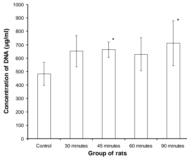
Figure 3. LMW DNA content in 10,000×g supernatant of testicular cells after various continuous heat treatment at 43° C in various animal groups. Data presented as mean ± SD from 6 observations. *: p \leq 0.05 when various heat -treated animals compared to control counterparts. Mean value is in µg/ml of 10,000×g supernatants
