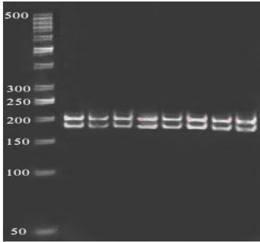
Figure 3. Fragments (12, 181, 198 bp) of HinPII enzyme digestion of amplified exon 5 (391 bp) on 2% polyacrylamide gel in 80 constant voltage in RFLP method. 50 bp ladder was used (polyacrylamide gel was used to identify more exactly between fragments)
