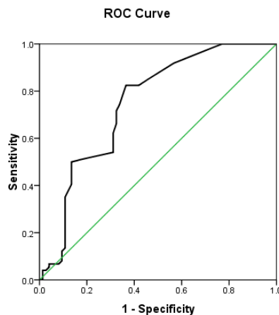
Figure 1. ROC curves for AST for the detection of PPRM. The area under ROC curve was 0.747. Diagonal segments are produced by ties.
