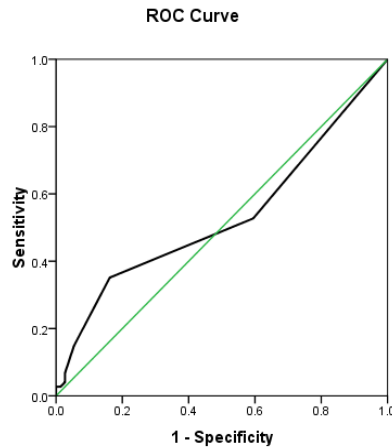
Figure 2. ROC curves for ALT for the detection of PPROM. The area under ROC curve was 0.53
