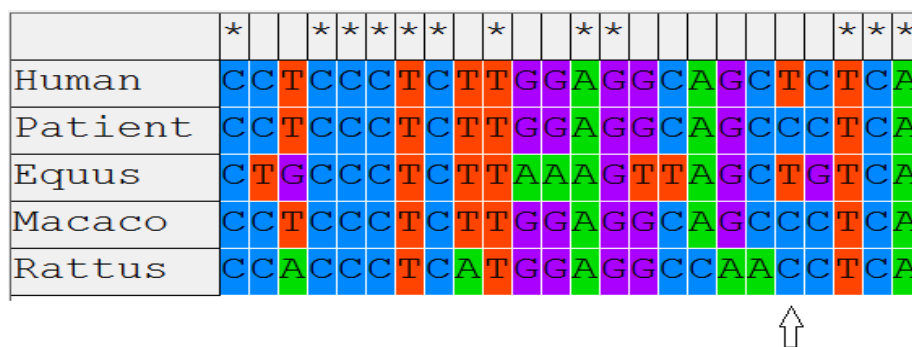
Figure 2. Multiple sequence alignment of g.IVS1+75T>C mutation in TNPI gene of human with other species and the arrow (*) indicate the sites of this mutation.
