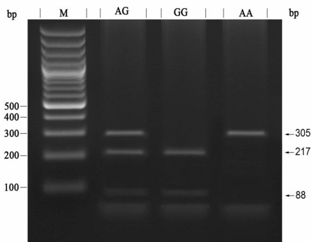
Figure 1. Identification of polymorphism at position A919G after digestion with AhdI restriction enzyme. M: DNA Marker, AG: Heterozygous genotype digested to three fragments (305bp, 217bp, 88bp), GG: Homozygous for G allele digested to two fragments (217bp, 88bp), AA: Homozygous for A allele with no digestion
